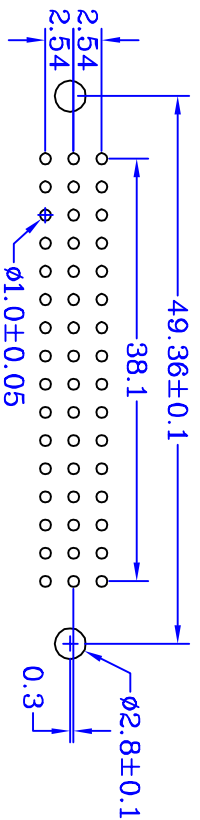
PCB LAYOUT
